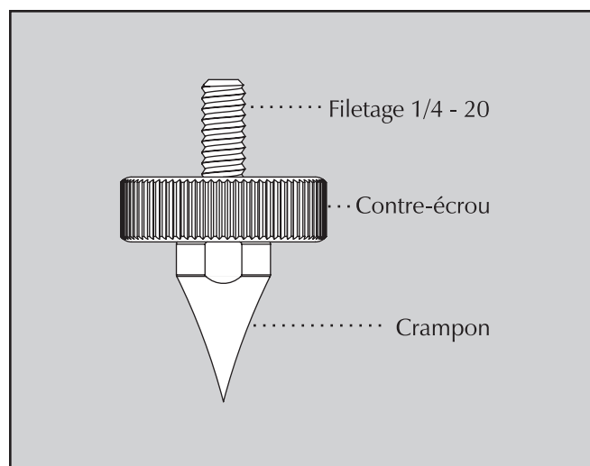
Figure 7. Le crampon ETC
